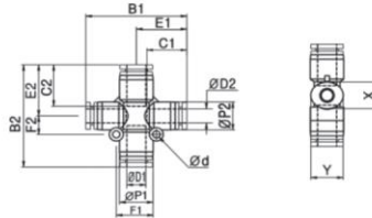
MODEL[ØD-T] Tube(Inch)–Thread(NPT)
