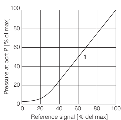
1 Regulation diagrams with flow rate Q = 10 l/min
